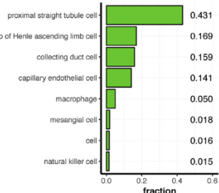
J microwell
