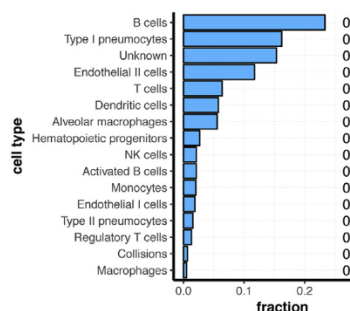
A sci-ATAC-seq
