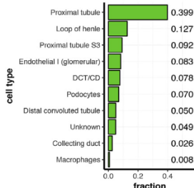
H sci-ATAC-seq
