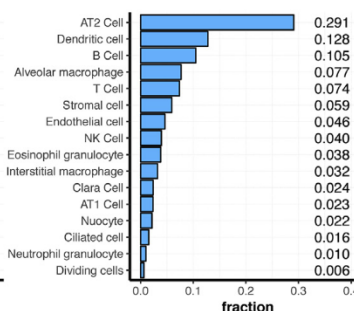
B microwell
