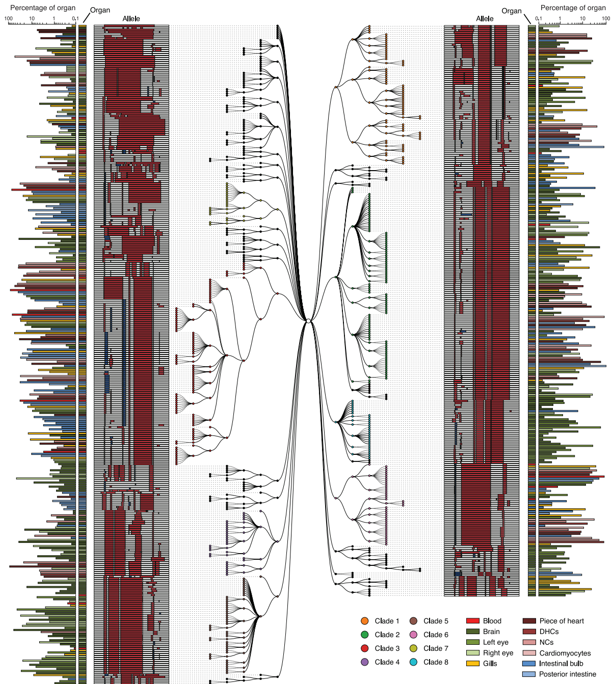
Fig. 6. Lineage reconstruction for adult zebrafish ADRL. Unique alleles sequenced from adult zebrafish organs can be related to one another using a maximum parsimony approach implemented in the PHYLIP Mix package (see Materials and Methods and fig. S4B). For reasons of space, we show a tree reconstructed from the 601 ADRL alleles observed at least five times in individual organs. Eight major clades are displayed with colored nodes, each defined by
