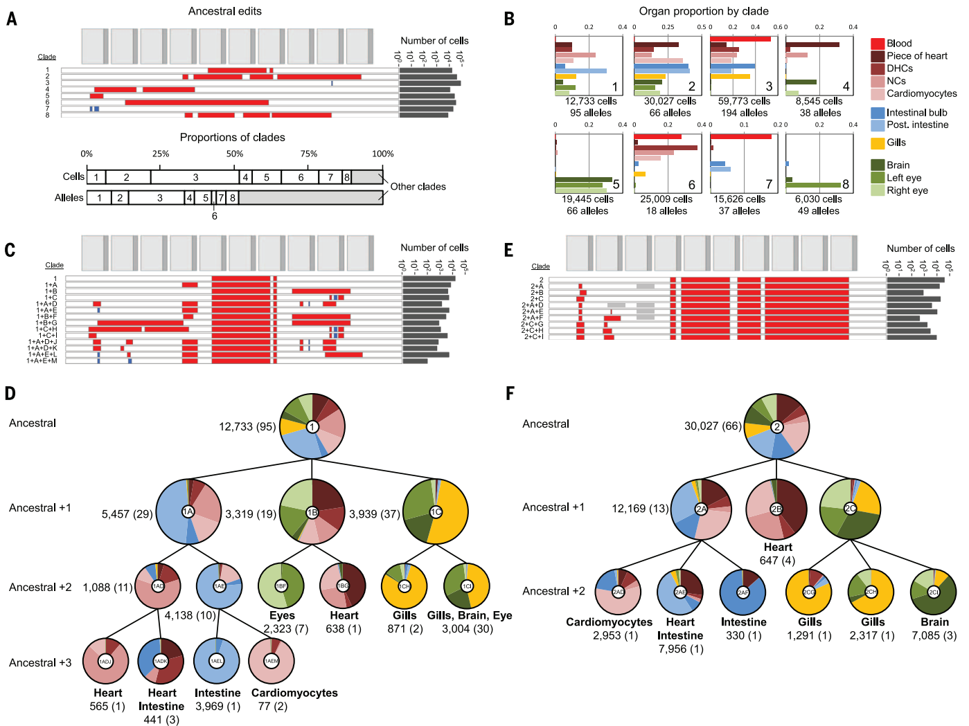
Fig. 7. Clades and subclades corresponding to inferred progenitors exhibit increasing levels of organ restriction.
